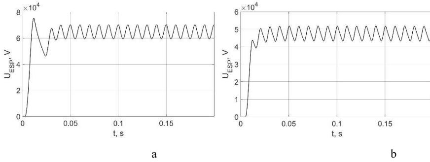
Fig. 6. Voltage at the ESP input at firing angles: a – 45°; b – 90°.
