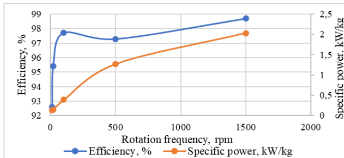
Fig. 3. Dependence of efficiency and specific power on the rotational speed.
