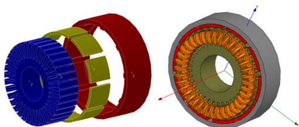
Fig. 2. Permanent magnet synchronous generator with external rotor.
