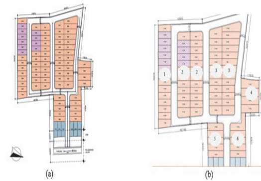
Fig. 3. (a) Building unit plans at residential locations (b) Tributary area for channel planning.
