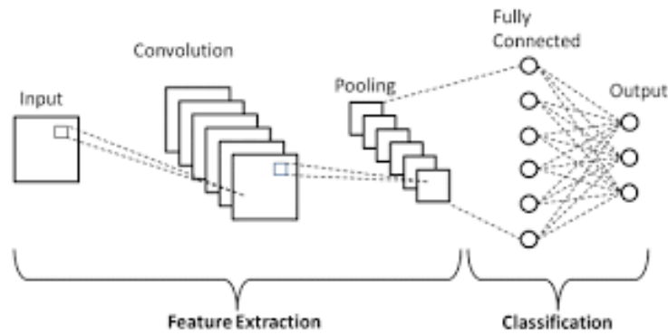
Fig 7. CNN Model
