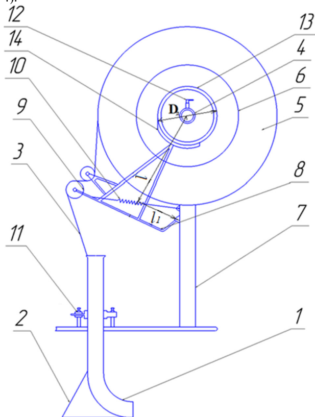
Fig. 4. The design of the drip tape stacker with a brake device: 1 - guide pipe, 2 - coultter, 3 - drip tape, 4 - shaft, 5 - drip tape reel, 6 - pressure disc, 7 - vertical support column, 8 - brake device, 9 - tension roller, 10 - spring, 11 - laying depth adjuster, 12 - disc retainer, 13 - disc rim, 14 - block.
