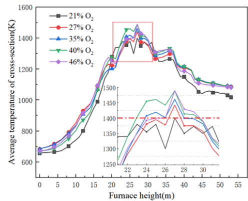
Fig.3 The temperature changes along the height.
