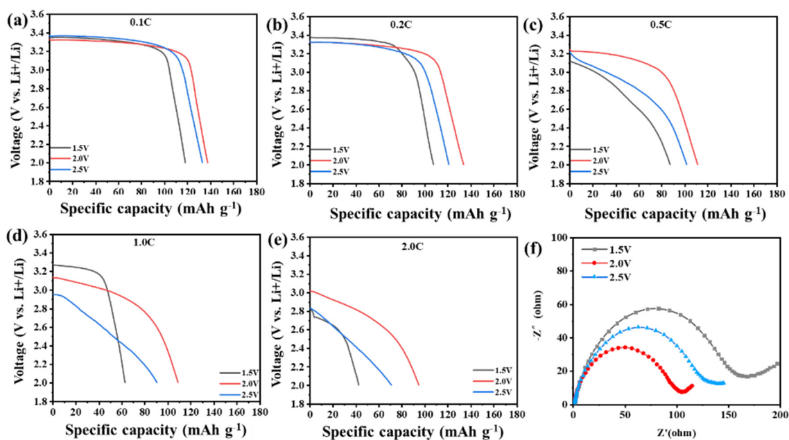
Fig. 4 The discharge capacity curves of LiFePO 4 after delithiation at different voltages. (a) 0.1 C; (b) 0.2 C; (c) 0.5 C; (d) 1.0 C; (e) 2.0 C; (f) Corresponding EIS curves.
