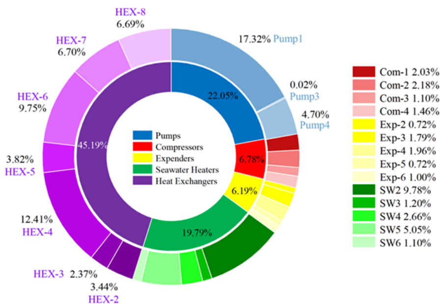
Fig.3 Energy loss of the device in the off-peak/medium-peak time
