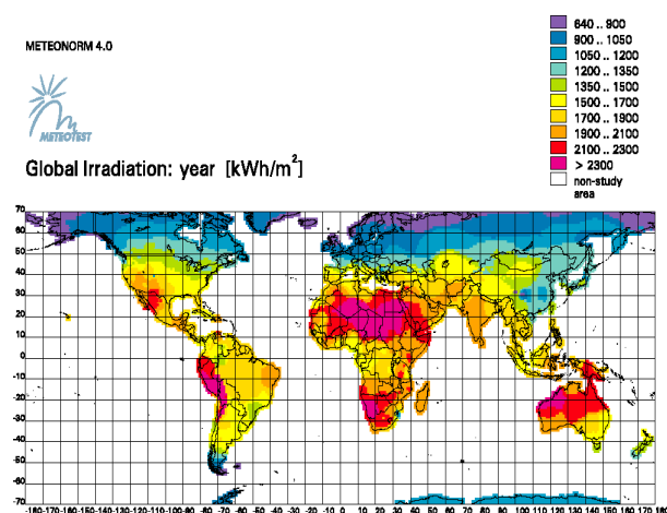
Fig. 7. Map of global solar radiation
