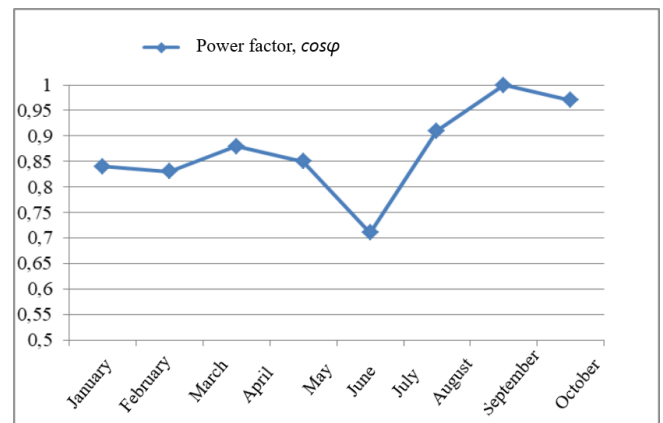
Fig.4. Power factor of Boiler-1
