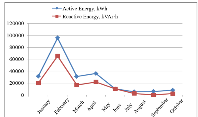
Fig.3. Dynamics of electricity consumption at Boiler-1
