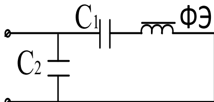
Fig.3. Series ferroresonant circuit with capacitor connected in parallel
