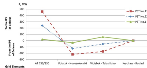
Fig. 3. Active power flow profiles along the 330 kV transmission line and the 750/330 kV AT of the IPS of Belarus with different taps of the PST selected in the maintenance state (disconnection of the 330 kV Krychaw-Roslavl overhead line).
