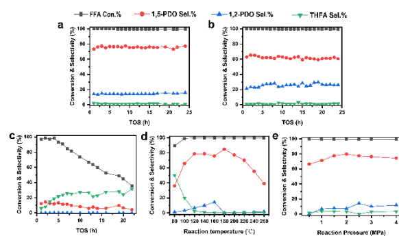
Figure 4. Catalyst performance test of (a) Cu-MFI (60)-AE, (b) Cu-MFI (130)-AE, (c) Cu-MFI(Si)-AE, 160 °C, 2.5 MPa H 2 . (d) catalyst performance test at different reaction temperature. (e) catalyst performance test at different H 2 pressure.
