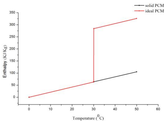
Fig. 3 Enthalpy-temperature curves of Two Models
