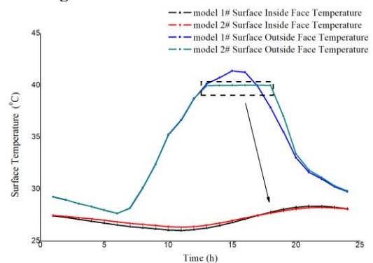
Fig. 10 Vary of surface temperature of two models
