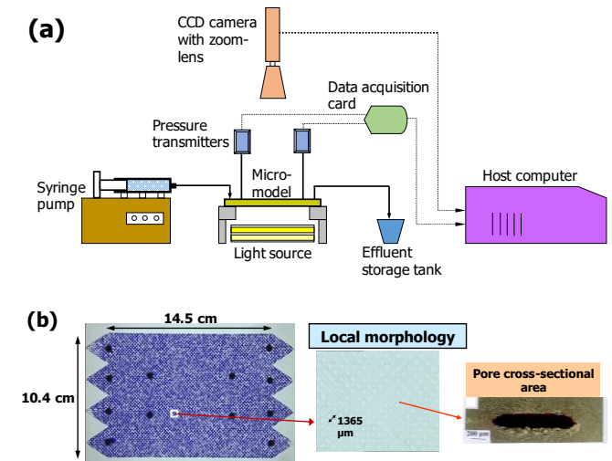
Fig. 2. (a) Schematic diagram of experimental setup. (b) Morphology of glass-etched pore network model.
