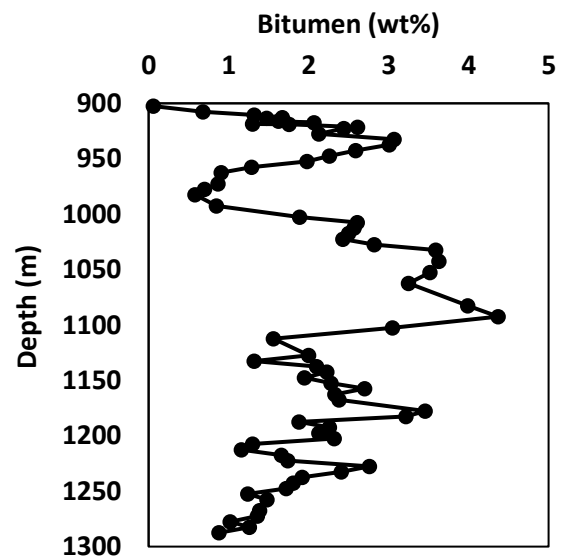
Fig. 5: Bitumen (wt%) with depth for the NESS 2 well as determined by Soxhlet extraction.
