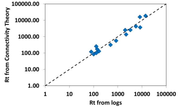
Fig. 8: Resistivity from NESS 5 well log from 1050-1056m versus resistivity calculated using the connectivity theory model, with \chi_w = 0.03 and \mu = 2 .
