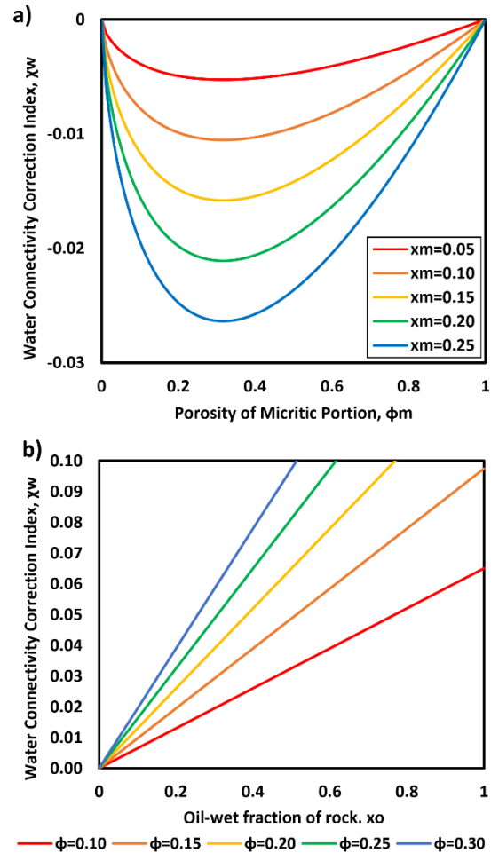
Fig. 2: a) \chi_w for a micritic portion of the rock in which \mu_m is 1.5 and \mu is 2 in equation (4). b) \chi_w for a rock with oil-wet pore spaces in which S_{co} is 0.65 in equation (5). \phi is the porosity of the macro pore space.
