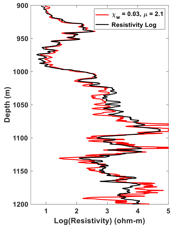
Fig. 9: Resistivity log from the NESS 2 well overlaid with the connectivity theory resistivity calculated from Eq. 3 using the dielectric log for S_w\phi , \chi_w = 0.03 , and \mu = 2.1 .
