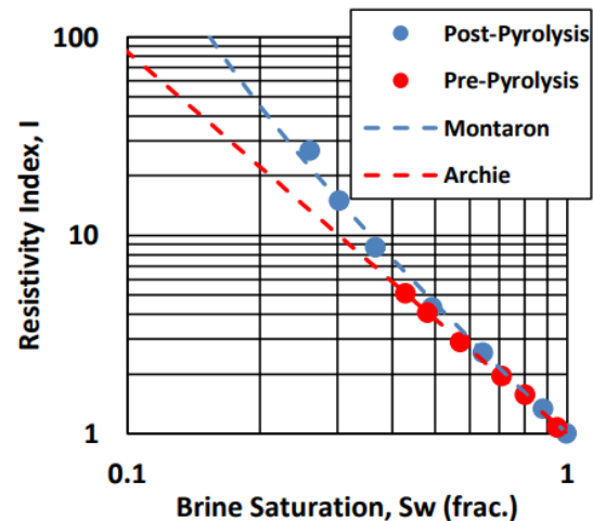
Fig. 1: Resistivity index versus brine saturation for an immature core sample from the Shefela basin pre- and post-pyrolysis [11].
