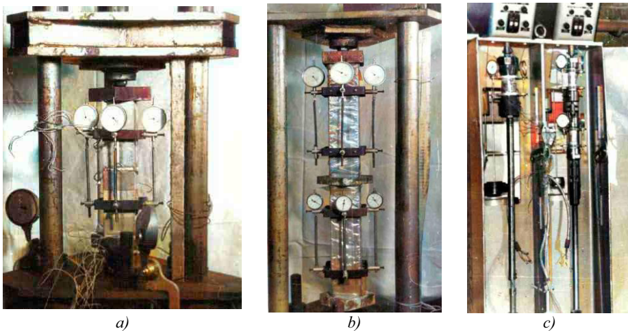
Fig. 3. Testing of specimens under long-term compression (a, b) and tension (c).
