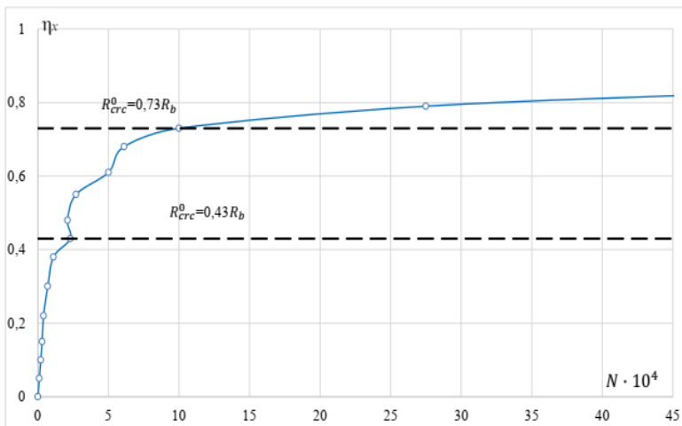
Fig. 8. Diagram "number of acoustic pulses vs. stress level in expanded clay concrete specimens"
