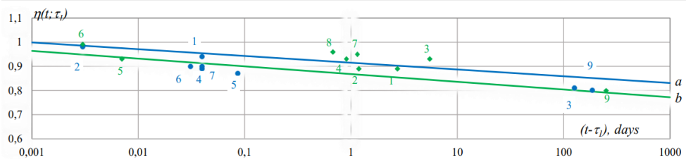
Fig. 9. Change in the long-term strength of expanded clay concrete over time under axial tension (a) and compression (b) by dependence (3)
