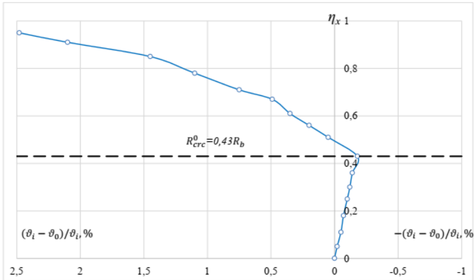
Fig. 6. Diagram "velocity of ultrasound transmission vs. stress level in expanded clay concrete specimens"
