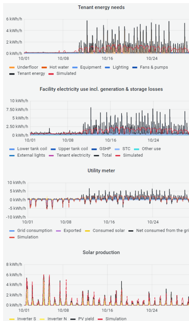
Figure 6 shows a screenshot from the observability platform presenting the model (red line) and detailed measurements of tenant energy needs, facility electricity use, net electricity consumption, and solar production per hour in October 2021.
