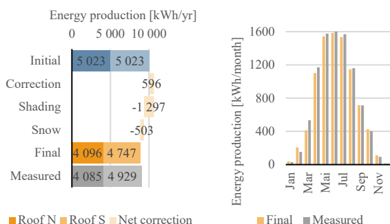
Figure 5 shows the total and monthly PV model for the initial model without accounting for site shading or snow effects, and the final model (orange) matches the measured values (grey).
