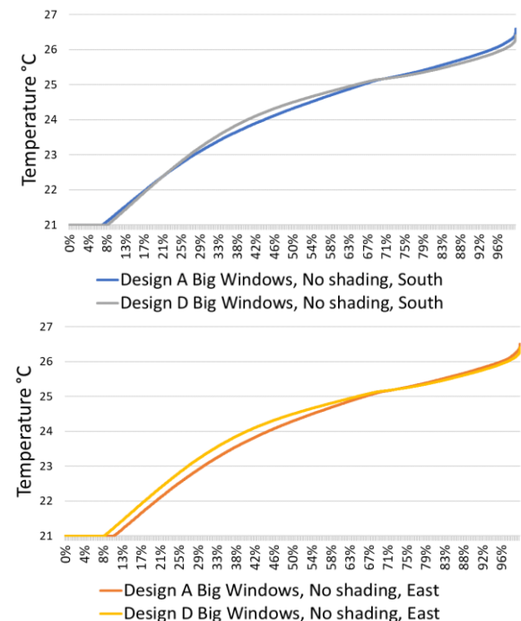
Figure 8: Duration curve for operative temperature in selected cases and offices, temperatures higher than 21 °C are presented only for difference magnification.
