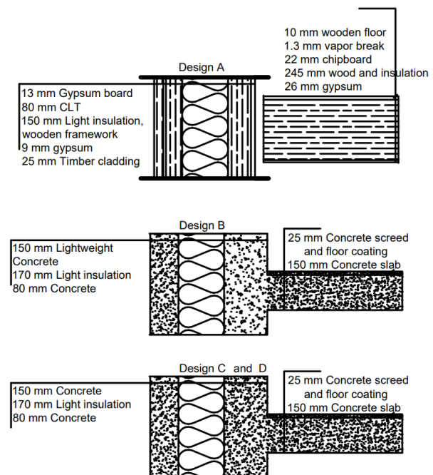
Figure 1: Structural design types of the case studies.
