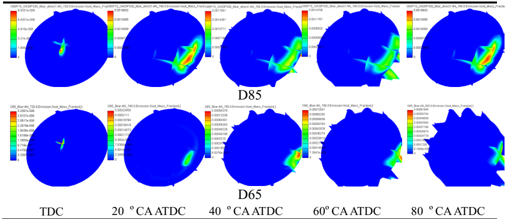
Fig. 13. The distribution of soot mass fraction in the cylinder with different DI/PI injection ratio.
