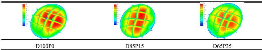
Fig. 8. Turbulent kinetic energy distribution in the cylinder at the moment of ignition.
