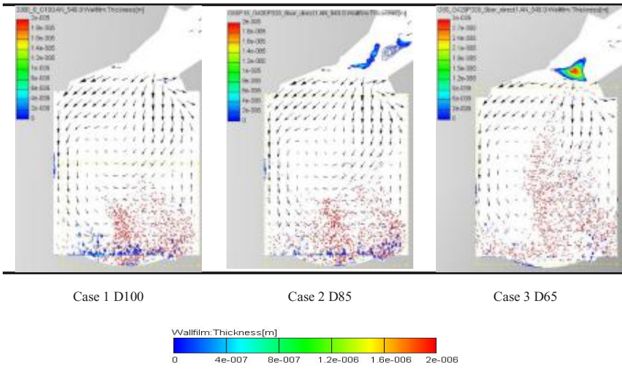
Fig. 5. The oil film in the cylinder at the intake valve close timing(549° CA).
