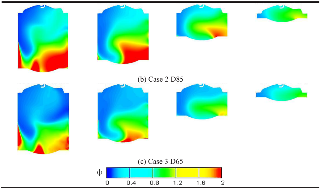
Fig. 4. Equivalent ratio of mixed gas in cylinder with different fuel injection ratio.
