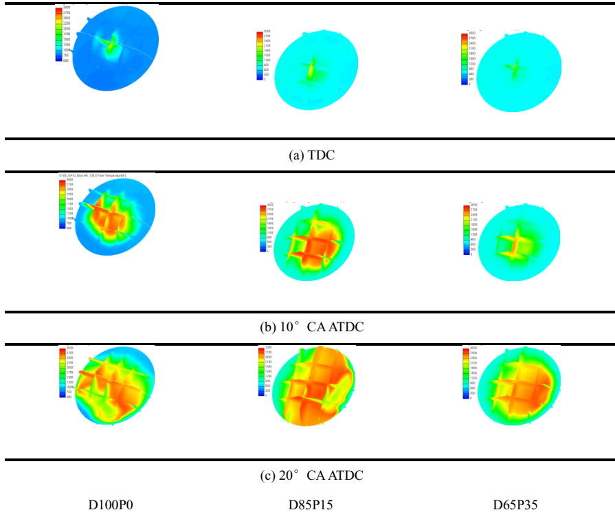
Fig. 10. Comparison of the temperature field in the cylinder with different fuel injection ratios.
