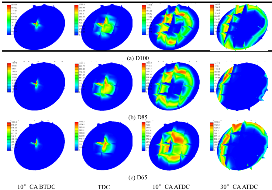
Fig. 9. Flame propagation process with different fuel injection ratios.
