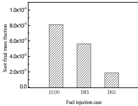
Fig. 12. The final mass fraction of soot in the cylinder with different fuel injection ratios.
