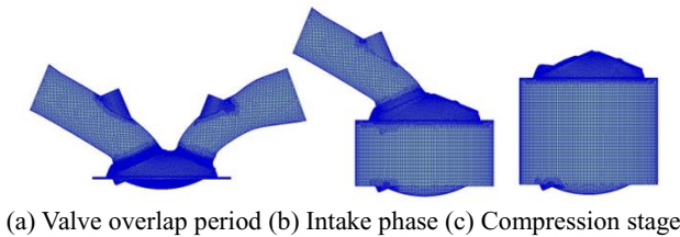
Fig. 2. Engine dynamic grid.
