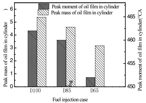
(b) Peak mass and peak moment of the oil film in the cylinder
