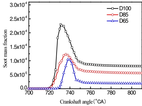
Fig. 11. Soot generation process in the cylinder with different DI/PI injection ratios
