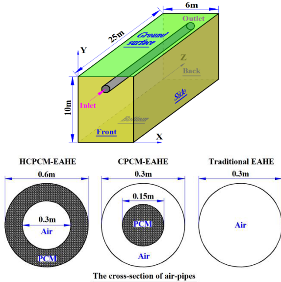
Fig.1 Schematic diagram and some key dimensions of HCPCM-EAHE, CPCM-EAHE and Traditional EAHE.
