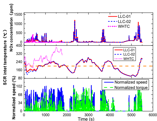
Figure 6 NO x transient emission characteristics of hot WHTC
