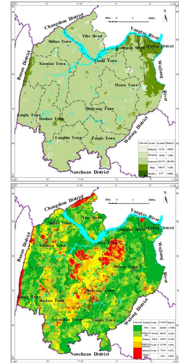
Figure 2 Evaluation map of Se and Zn abundance and deficiency in topsoil of the study area
