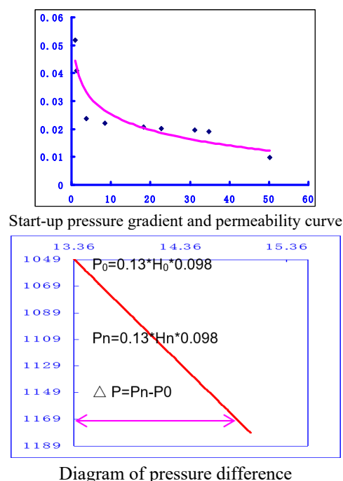
Fig.1 Start-up pressure gradient and permeability curve and
