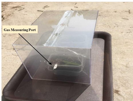
Fig. 1. Simulation box of roof greening air purification test
