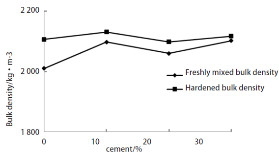
Figure 2. The influence of cement content change on the bulk density of desulfurized gypsum-based mortar
