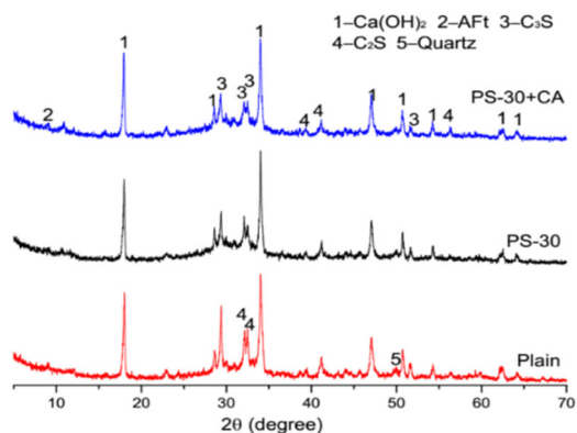
Figure 4. XRD pattern of hardened cementitious material
