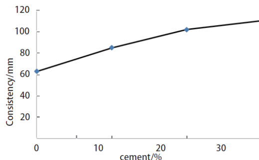
Figure 1. The effect of cement content change on the consistency of sulphurised gypsum-based mortar
