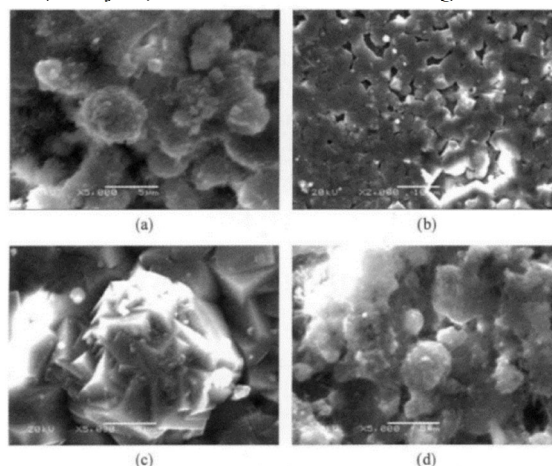
Figure 3. SEM image of hardened gel material
