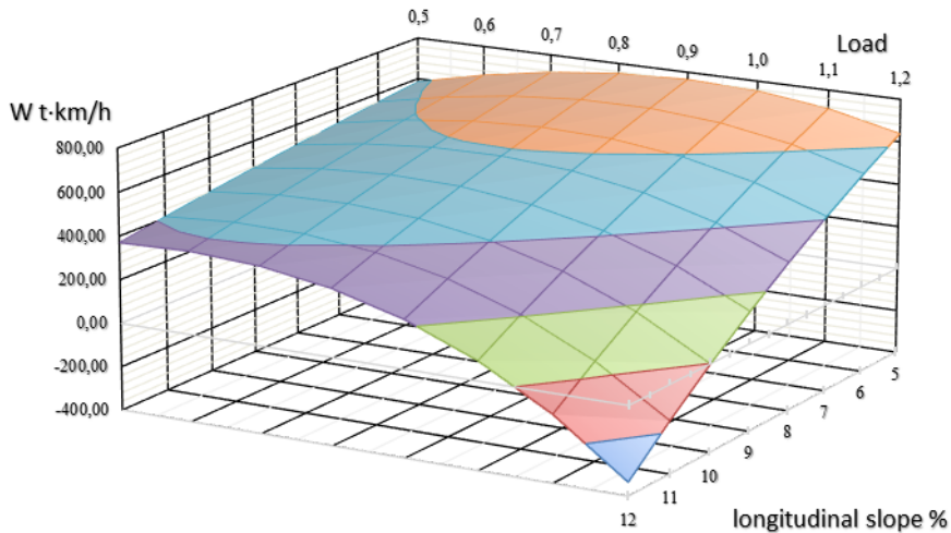
Fig. 6. The graphical dependence of the capacity ( W ) on the longitudinal slope ( i ) and the coefficient load capacity use ( \gamma_r ) at the ambient temperature of 40^\circ\text{C}
