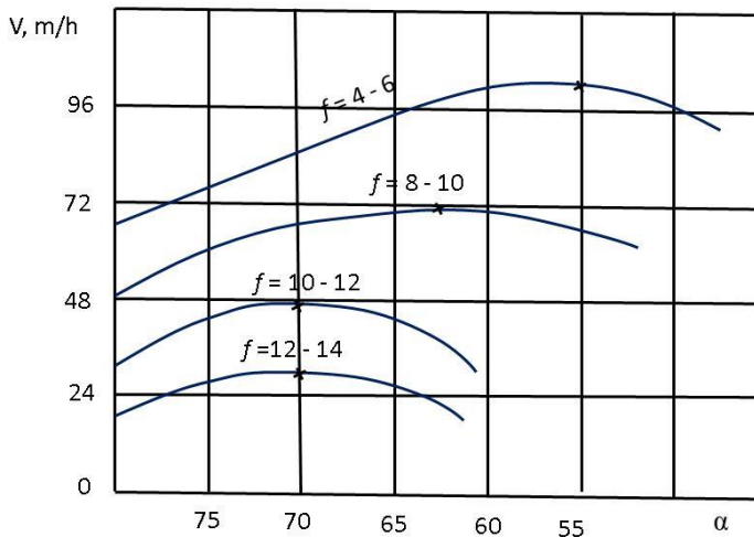
Fig. 3. Influence of the angle of sharpening of the drill bit on the productivity of drilling holes ( P = 1500 kg, n = 275 min -1 .)
