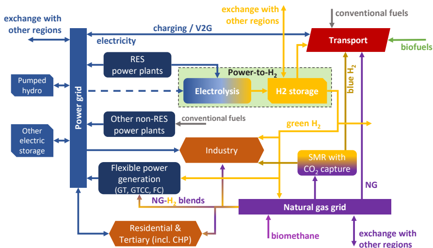
Fig. 1. Schematic of the energy connections within one node of the modelled energy system.
