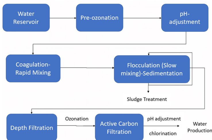
Figure 4. A typical flow chart of conventional water treatment processes.
