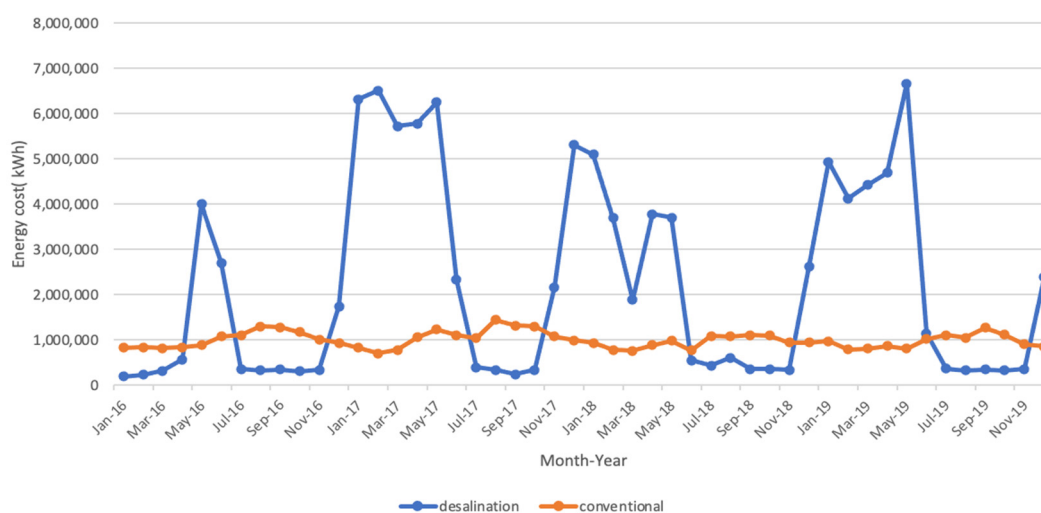
Figure 3. The relationship between energy consumption and seasonal change from conventional and desalination water supply systems
