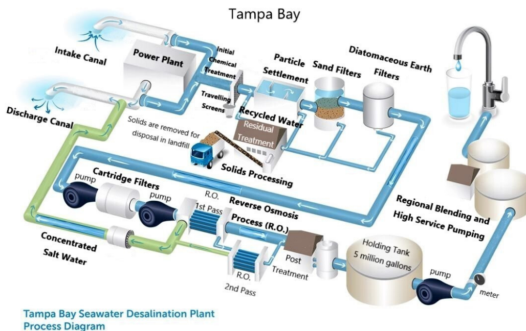
Figure 6. Diagram of Tampa Bay Seawater Desalination Plant Process 25
