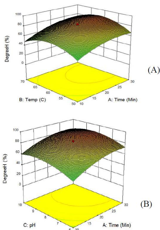
Fig.1. The 3-D surface plot of interaction between the parameters on degree of hydrolysis, (A) temperature and time, (B) pH and time.
