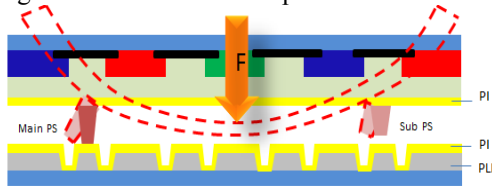
Fig. 3. Schematic diagram of PS extrusion test.
