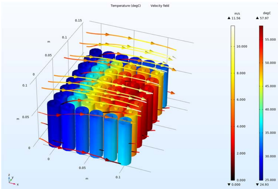
Fig. 4. Cloud map of temperature distribution.
