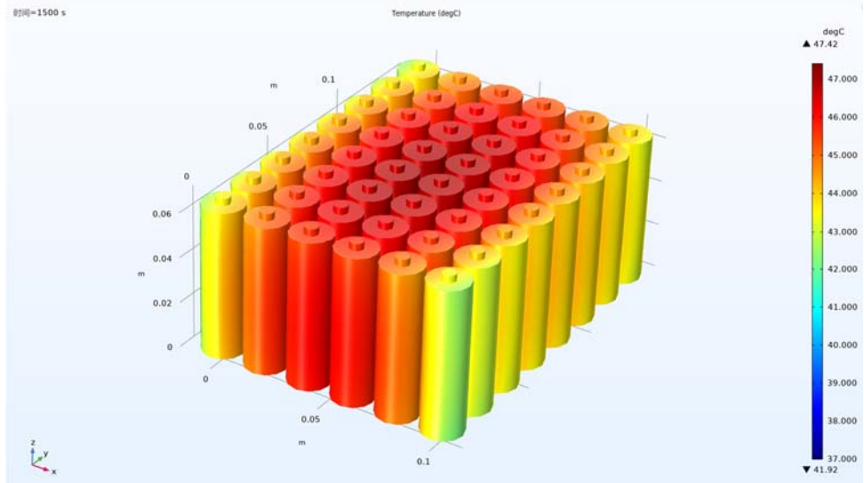
Fig. 5. Cloud map of temperature distribution.
