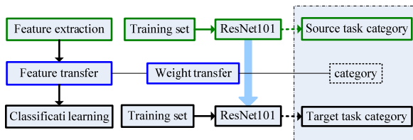
Fig. 2. Schematic diagram of transfer learning.
