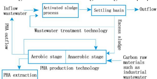
Fig. 3. Process flow model of PHA production by anaerobic-aerobic activated sludge [16]
