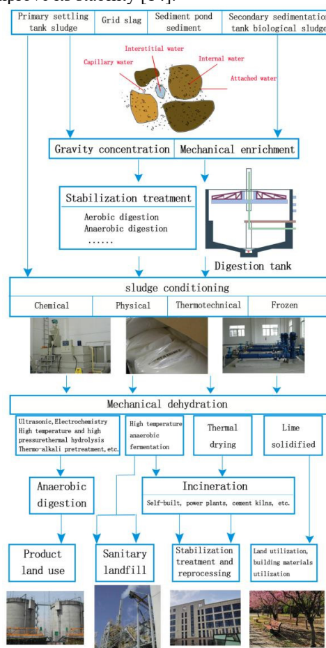
Fig. 1. The main process routes of sludge disposal in China [13]
