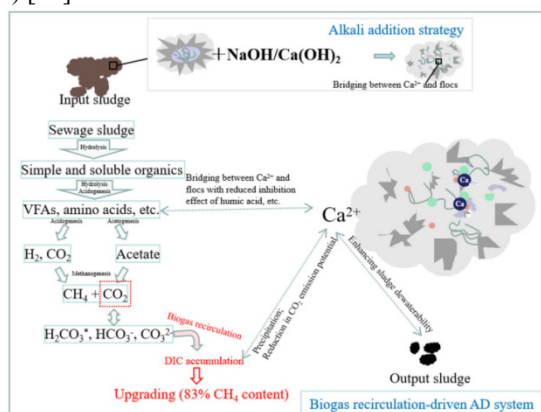
Fig. 2. The strategy of adding lye to the AD system driven by biogas recirculation for sludge management [14]
