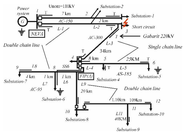
Fig. 1. Diagram of a 110 kV electrical network with a complex configuration (ES - electric power system; Substation -1, Substation -2, Substation -3, Substation -4, Substation -5, Substation -6, Substation -7, Substation -8 - consumer substations; L1, L2, L6, L7, L8, L9 - double-circuit 110 kV transmission line with P110-6 and PB-110-6 supports with one lightning cable and without them in separate sections; L3 - 110 kV single-circuit power line with P220-3 and PB-220-1 supports with and without a lightning cable in separate sections; L4, L5 - 110 kV single-circuit power line with P110-5 and PB-110-5 supports with or without a lightning cable in separate sections; T - lightning protection cable; K - short circuit point; 1, 2, 3, 4, 5, 6, 7, 8, 9, 10 - nodes of the electrical network; GN - grounded neutral).
