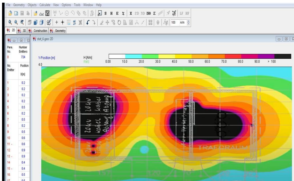
Fig. 3. Magnetic field
