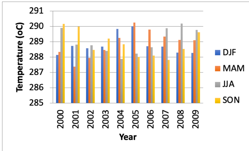
Fig.4. Seasonal temperature analysis between 2000-2009
