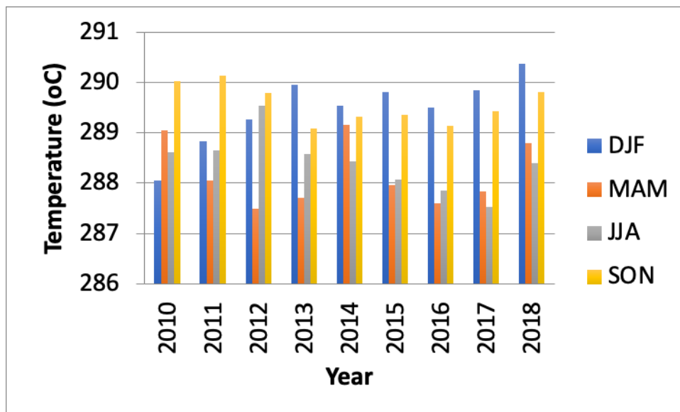
Fig.5. Seasonal temperature analysis between 2010-2018
