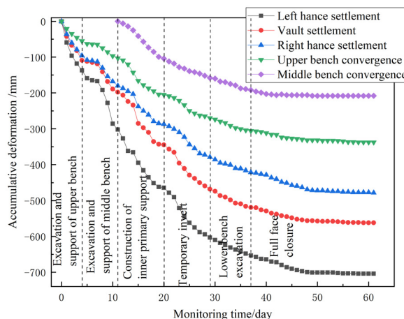
Fig. 10. Convergence Duration Curve of Section ZK40+991
