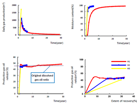
Fig. 2 Numerical simulation results of different permeability
