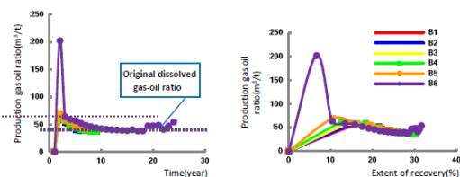
Fig. 5 Numerical simulation results of different flow pressures (formation low pressure)
