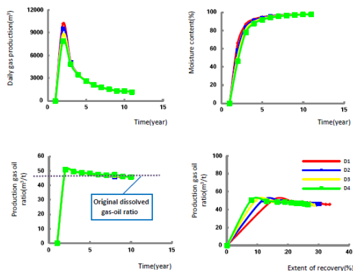
Fig. 3 Numerical simulation results of different oil viscosities
