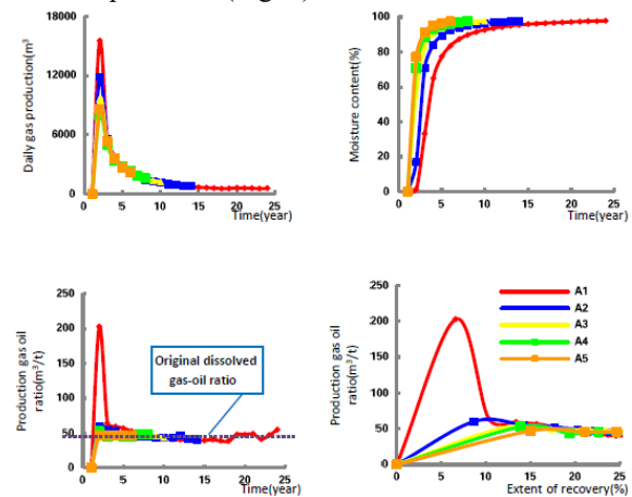
Fig. 4 Numerical simulation results for different formation pressures
