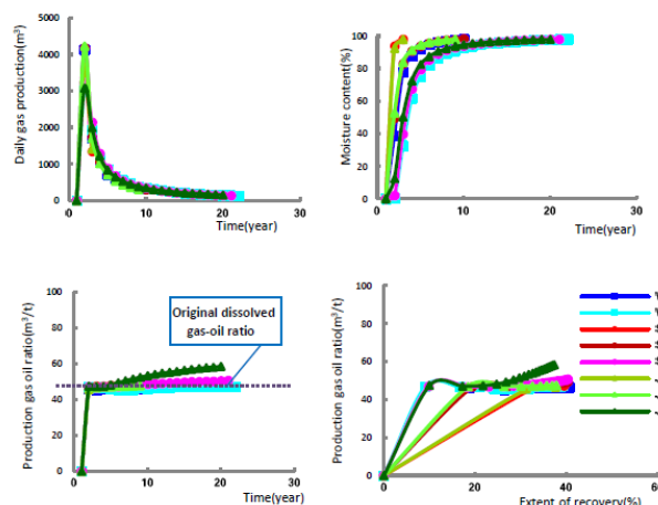
Fig. 7 Numerical simulation results of different well patterns and well spacing
