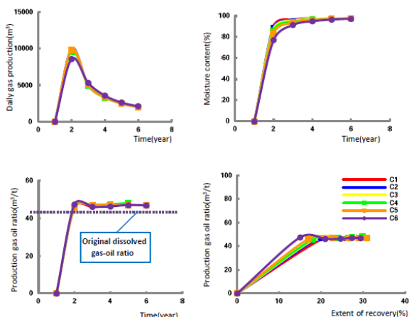
Fig. 6 Numerical simulation results of different flow pressures (formation high pressure)
