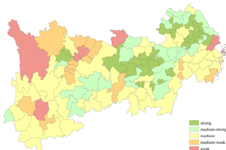
Fig.1 Results of groundwater resource carrying capacity in Yangtze River Economic Belt
