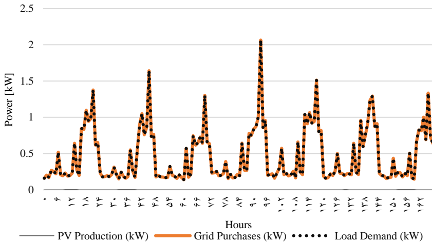
Fig. 4. The curve of system’s operation in terms of power sources for optimizer mode
