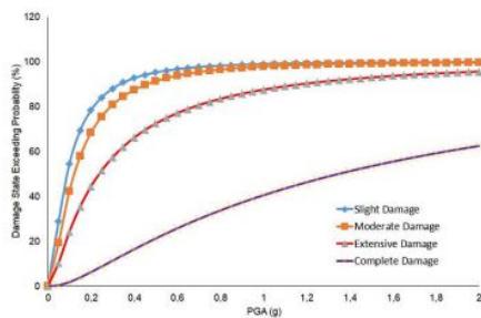
Fig. 3 Fragility curves of a cable-stayed bridge.
