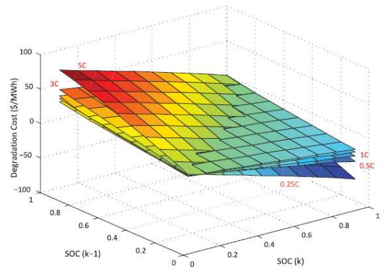
Figure 4 Cycle cost under different DOD and discharge efficiency Relationship curve with DOD
