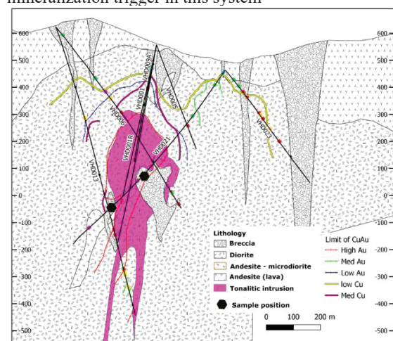
Fig 2. Interpretation of east-west section geological model of Huma Leu East and the sample described in this study.
