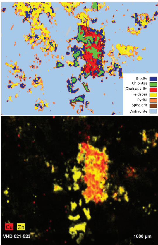
Fig 6. Distribution and association of chalcopyrite-sphalerite that's associated with biotite-chlorite-feldspar (picture analysis at position 2 of Fig 3c)
