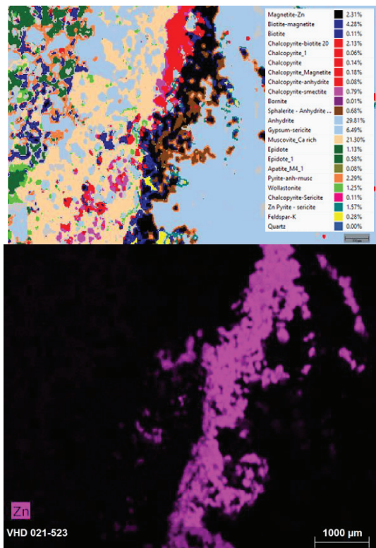
Fig 7. Distribution and association of chalcopyrite-magnetite-sphalerite that's associated with biotite-chlorite-feldspar-sericite-epidote-anhydrite in contact of siliceous phase and sulfate phase (picture analysis at position 1 of Fig 3c)
