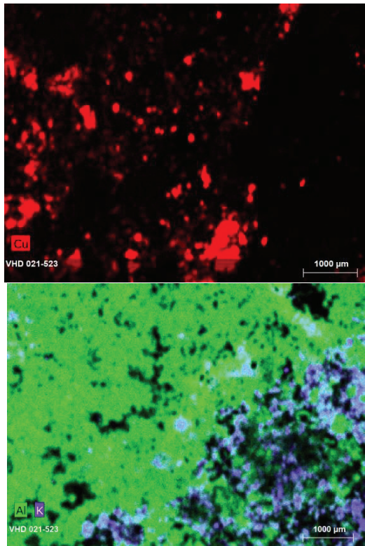
Fig. 4. The siliceous phase of cement breccia from sample VHD021/523 (at position 3 of Fig 3c), shows the distribution of copper minerals and related to Aluminopotassium minerals cement. (picture analysis at position 4 of Fig 3c),
