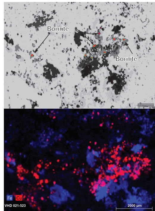
Fig 5. Distribution of bornite that's associated with chalcopyrite and feldspar. Table of point analysis shows object 1 as bornite with empirical formula as Cu_{3.6}FeS_2 , and the other was mix with feldspar minerals. (picture analysis at position 5 of Fig 3c)
