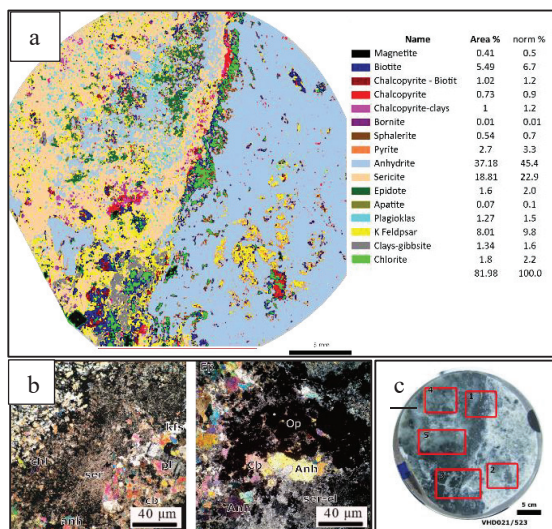
Fig 3. Mineralogical analysis of cement hydrothermal of sample VHD021/523. (a) A quantitative mineralogy from \mu -XRF data shows two dominant variation consist of calcium sulfate group in right side, silicate groups in left side, and also clays in bottom (b) petrographic analysis shows cement mineral, consist of quartz (qz), K Feldspar (kfs), plagioclase (pl), sericite (ser), anhydrite (anh), epidote (ep), carbonate (cb), chlorite (chl), clays (cl), an opaque (op), (d) polish section for \mu -XRF analysis and box position of detailed \mu -XRF analysis.
