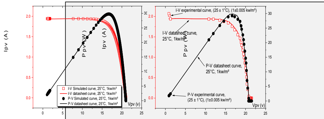
Fig. 7. I-V and P-V characteristics of the SX 330J module at 25 °C and G=1000\text{W/m}^2
