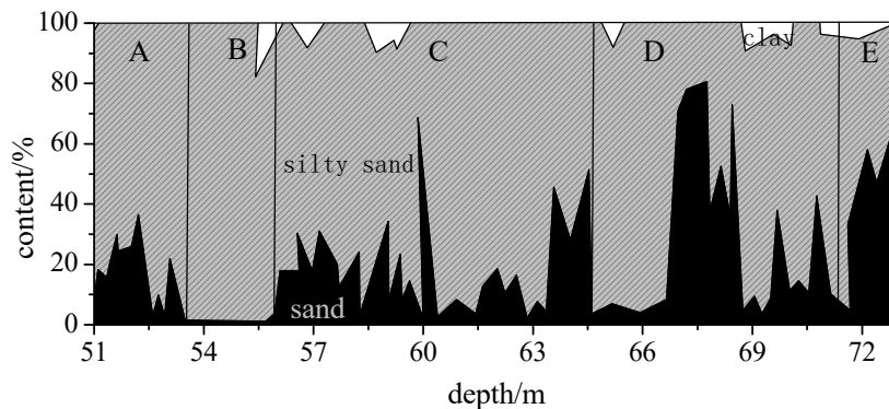
Fig. 1 Distribution and content of particles in 51~73m SG01 borehole
