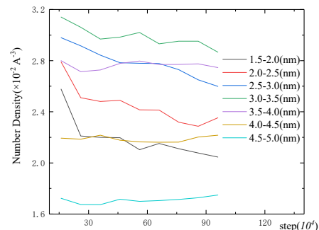
Figure 9. Number density of water around hydrophilic particle in the third stage vs. the step numbers.
