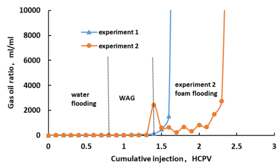
Fig 6. Gas oil ratio curve
