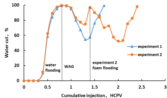
Fig 5. Water cut curve
