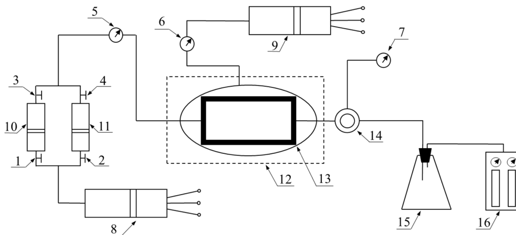
Fig 1. The experimental flow of gas breakthrough control in the planar model
