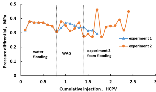
Fig 7. Pressure differential curve
