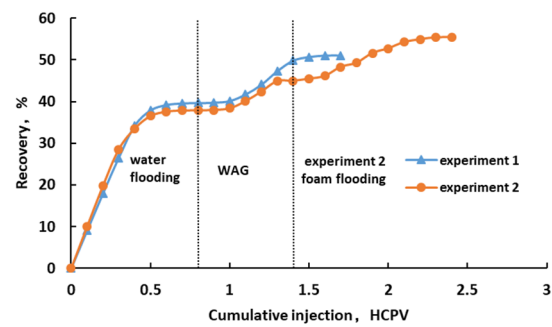
Fig 4. Recovery curve
