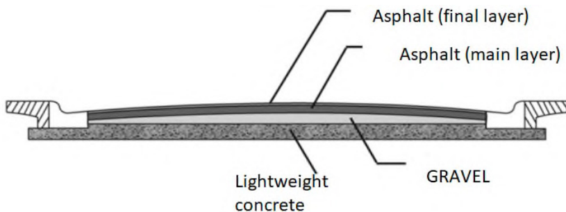
Fig. 1. Application of light concrete in road construction.
