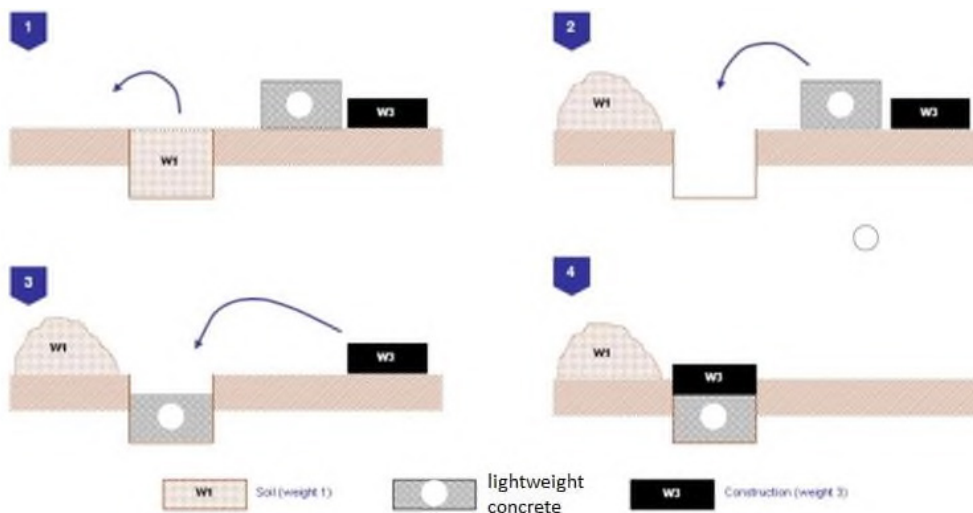
Fig. 2. The method of application of lightweight concrete in the construction of roads.
