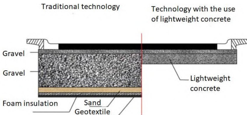
Fig. 3. Comparison of traditional road surface construction technology and light concrete technology.
